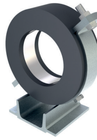
Type 171-1 H plus 1 piece with retaining profile incl. 2-phases active seal (no seal paste needed)
